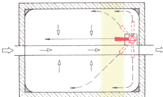
Fig. 5. Pivoting jet cleaner in a rectangular tank.
