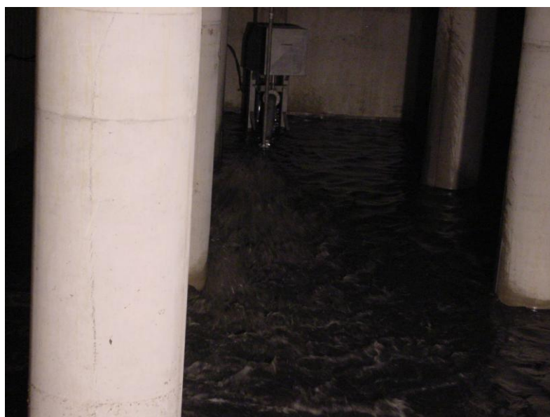
Fig. 9. Pivoting jet cleaner running.
