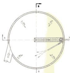
Fig. 6. Pivoting jet cleaner in a circular tank.
