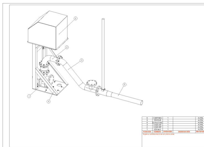
Fig. 3. Design of pivoting jet cleaner with diving bell.
